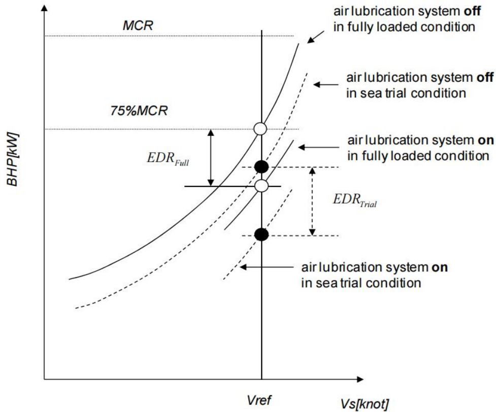
Figure 3.4.2 Prediction of the Reduction Rate of Propulsion Power due to Air lubrication and drag reduction system
