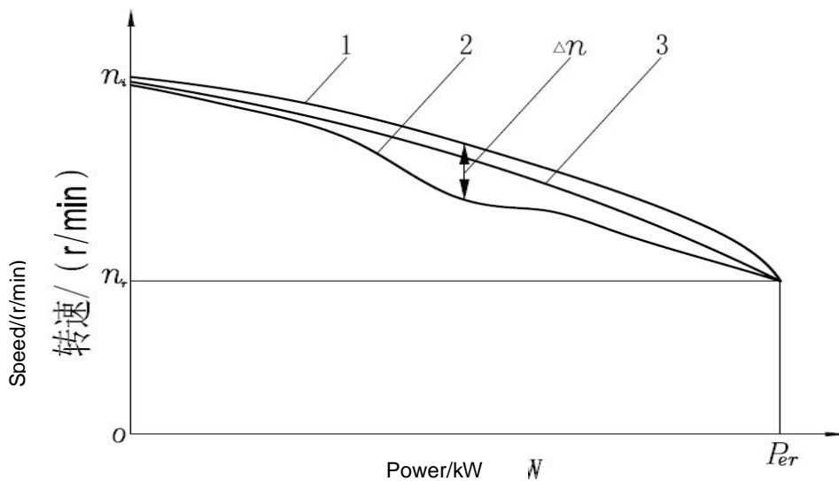
Fig. 3.2(168) Speed governing characteristic curve
