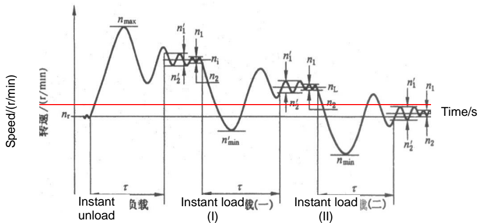
Fig. 3.2(2) Speed governing
