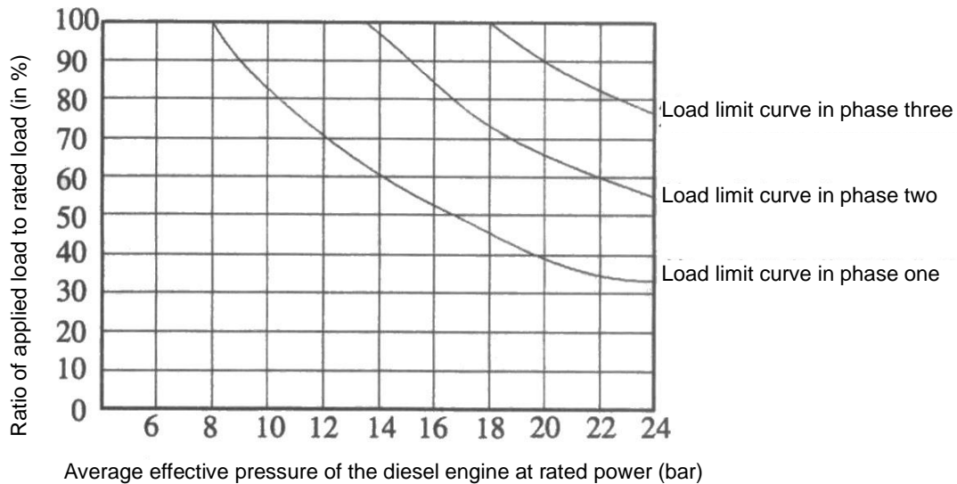
Fig. 7.5.6(1) Loading methods for the speed governing test of the highly supercharged four-stroke diesel engine
