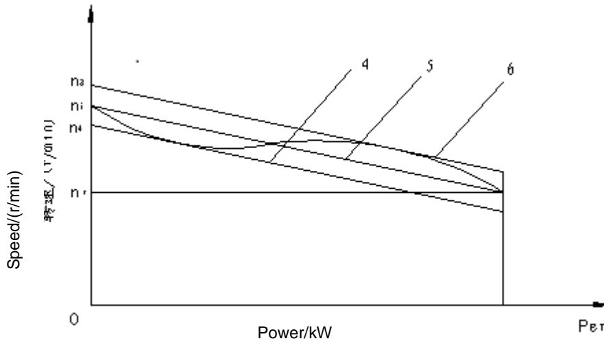
Fig. 3.2(180) Non-linearity of speed governing characteristic curve
