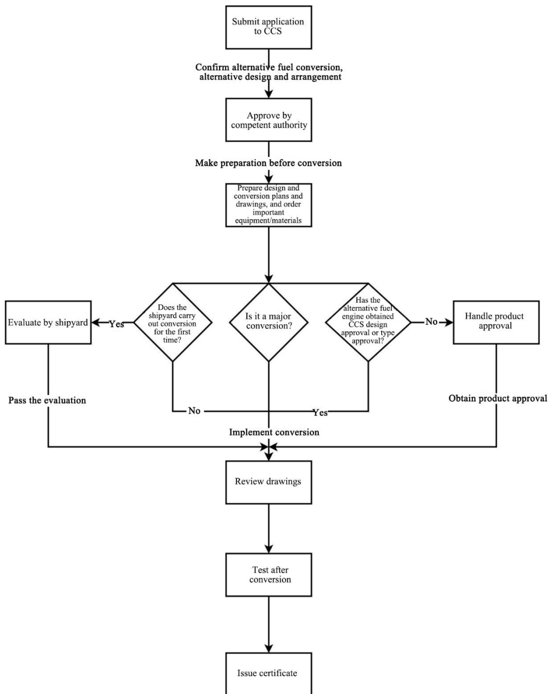
Figure 1.3.1 Conversion Process
