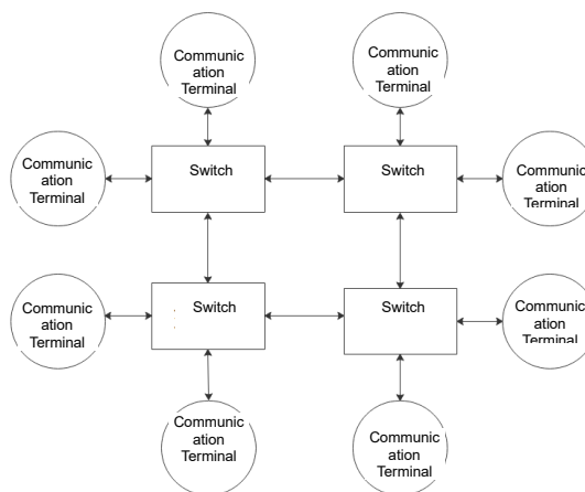
Figure 3-2.1.1(2) Ring Topology Diagram
