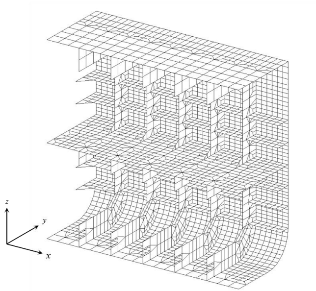
Figure 2.2.1.3 Schematic diagram of local structural member model
