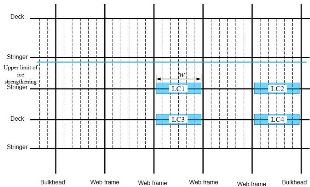
(a) Longitudinal member
