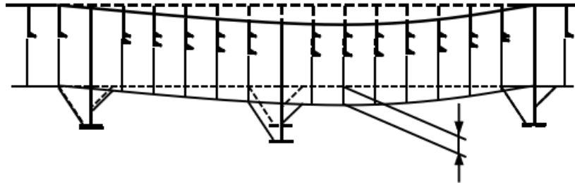
Figure 3.4.3(1) Measurement of displacement for lateral deformation
