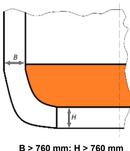
Figure 1: Permissible arrangement of a heavy fuel tank on board that meets the requirement of paragraph 4.4 of the draft guidelines or in accordance with regulation 12a of Annex I to MARPOL, if applicable
