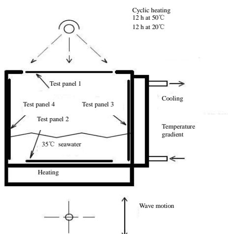
Fig. 1 Wave tank for ballast tank coating test
