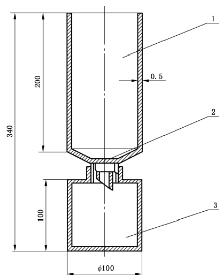
Fig. 8(2) Foam Receiver
