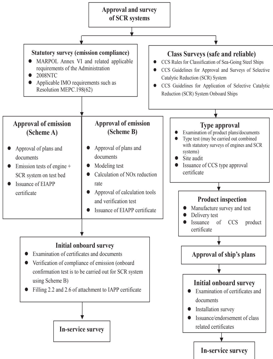
Related Procedures for Approval and Survey of SCR Systems
