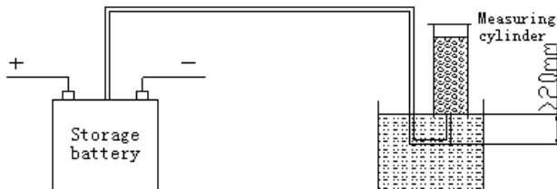
Figure 7.14 Gas collection
