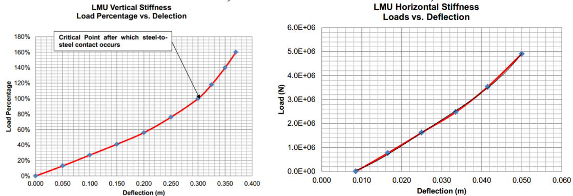
Figure 7.6.3 (3) Load-deformation Curve of LMU
