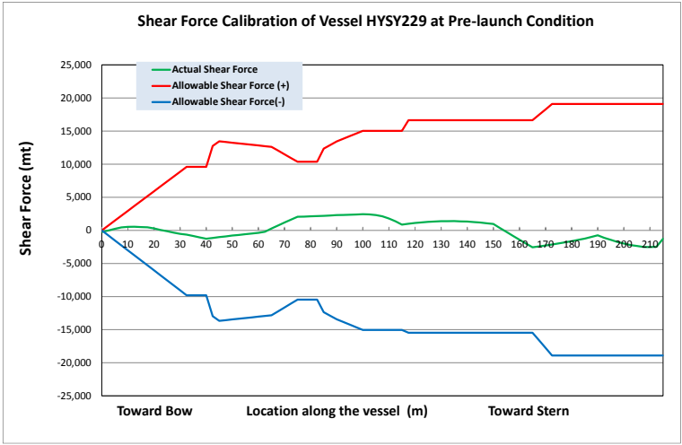
Figure 1.5 (4) Longitudinal Strength Check before Launching — Shear Force
