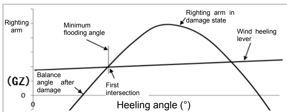
Fig. 4.3.2 Typical Hydrostatic Curves in Damage Condition
