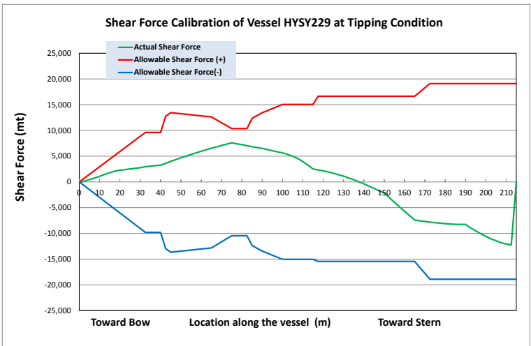
Figure 1.5 (6) Longitudinal Strength Check during Rotation — Shear Force
