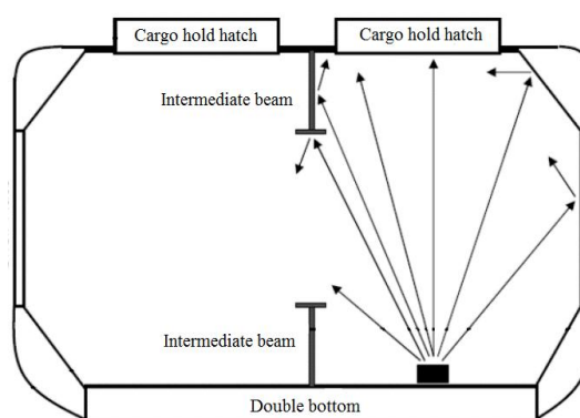
Figure 2 Cargo hold with intermediate beams
