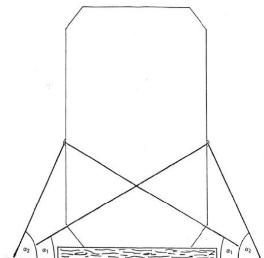
Figure 1 Principles of securing heavy items against sliding and tipping
