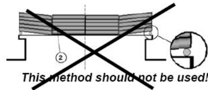
Figure 6.8 Principles for friction securing of round wood in restricted sea areas
