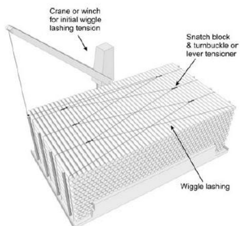
Figure 2.3. Example of wiggle lashings
