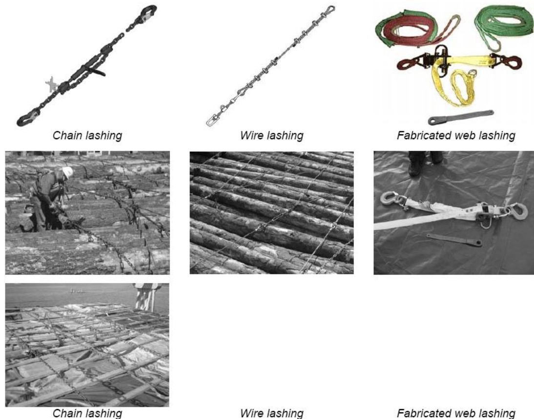
Figure 2.1 – Examples of different types of lashing equipment
