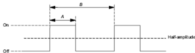
Figure 6 Typical modulation waveform
