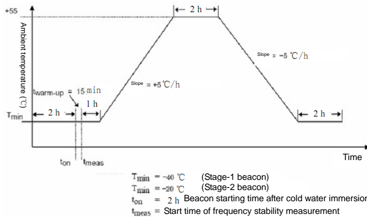
Figure 5 Temperature gradient
