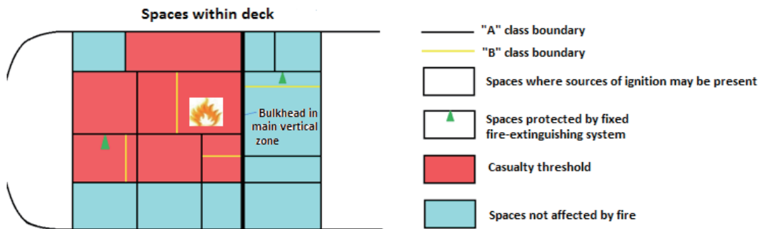
Figure 1.5.2(4) Not protected by fixed fire-extinguishing system (main vertical zone)
