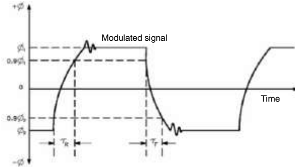
Figure 3 Definition of Modulated Rise and Fall time
