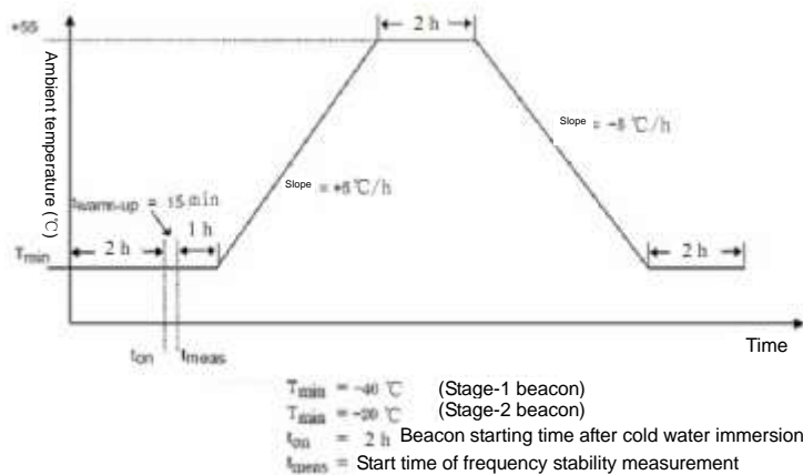
Figure 5 Temperature gradient
