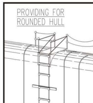
Figure 4.1 Pilot ladders
