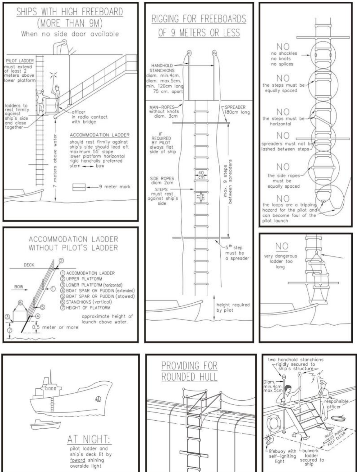
Figure 4.1 Pilot ladders
