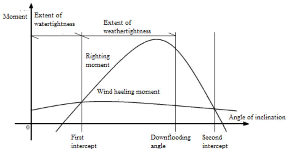
Fig. 2.4.2.1 (1) Typical Hydrostatic Curves in Damage Condition
