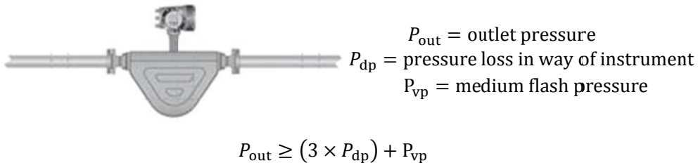
Figure 2 Pressure of Flowmeter
