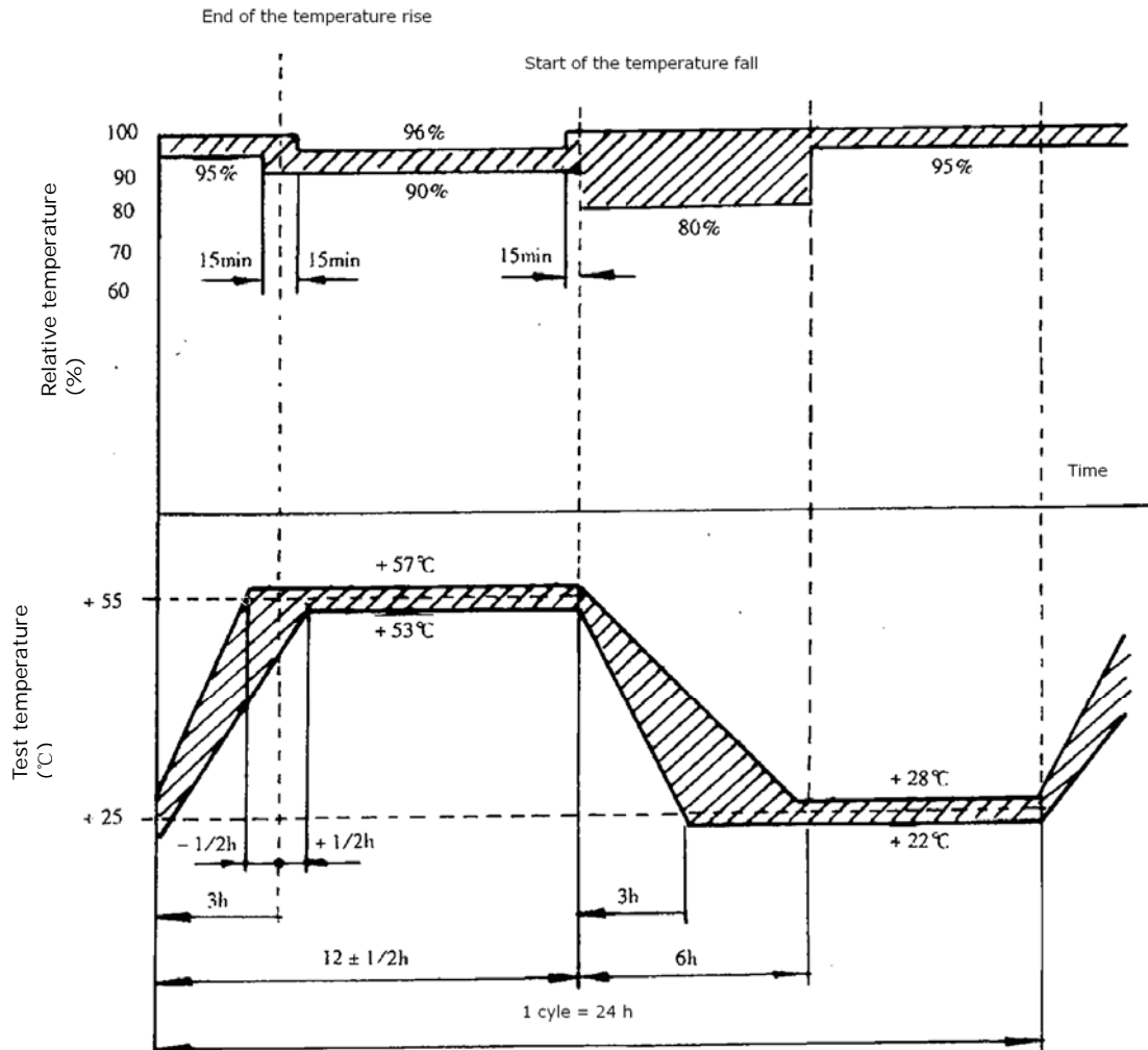
Figure 2.10.4.1(3) Test cycle
