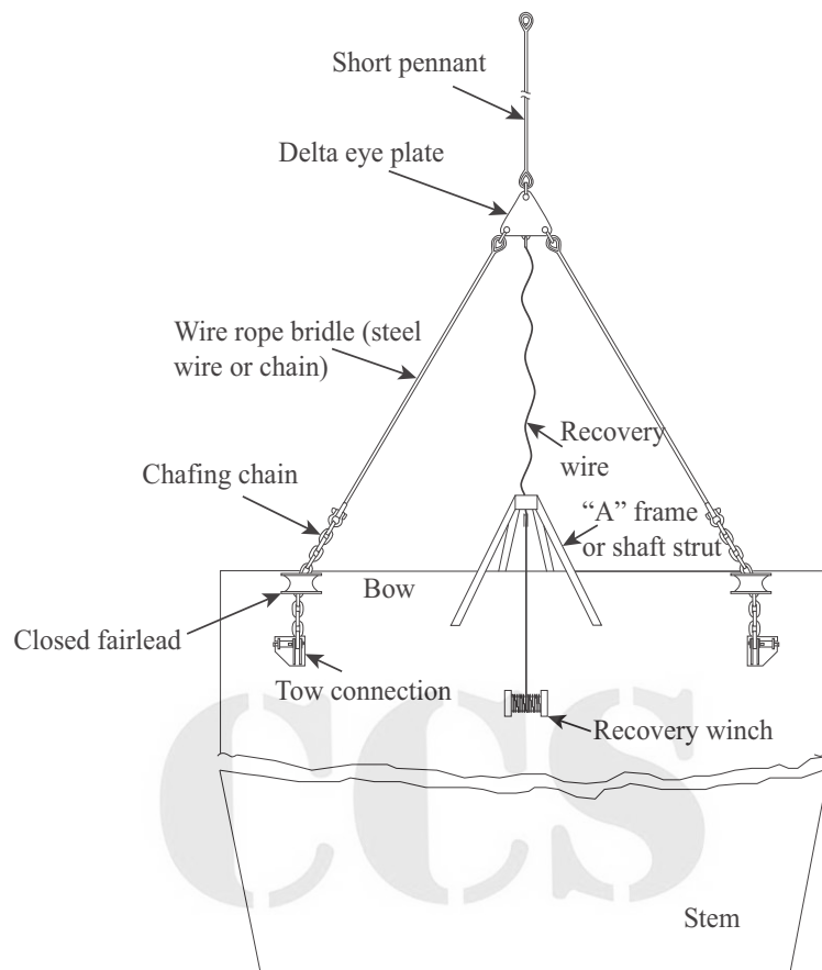
Figure 5.3.13 Arrangement of wire rope bridle/chain bridle recovery system
