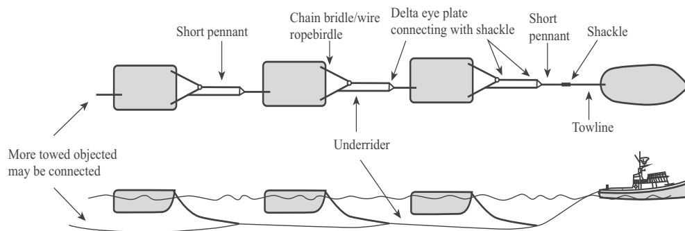
Figure 1.3 Diagram of parallel tow
