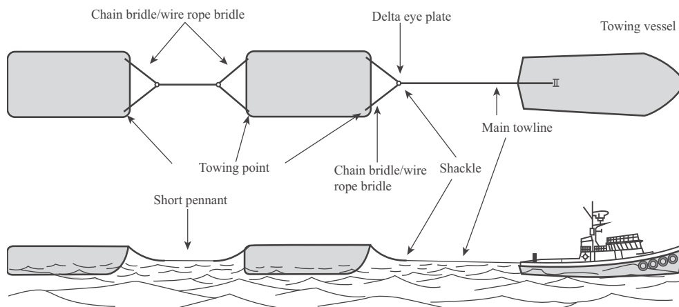
Figure 1.2 Diagram of tandem tow
