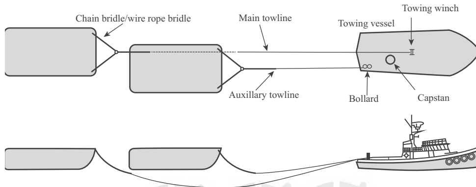
Figure 1.1 Diagram of double tow
