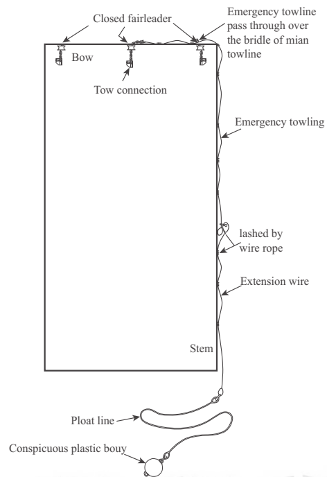
Figure 5.3.16 Arrangement of emergency towline on towed object normally unattended
