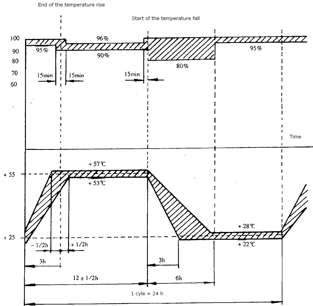
Figure 2.10.4.1(3) Test cycle
