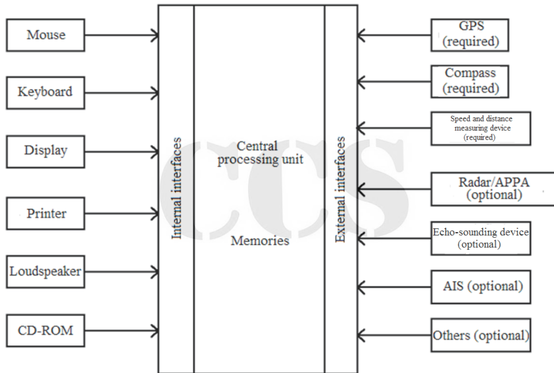
Figure 2.1.2 ECDIS System
