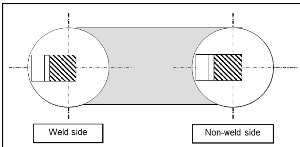
Figure 1 Location of CTOD test specimens for chain
