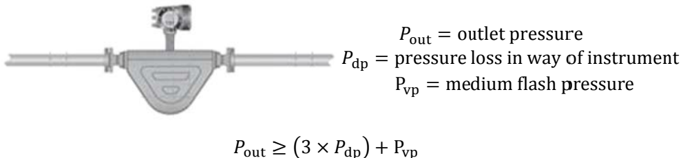
Figure 2 Pressure of Flowmeter
