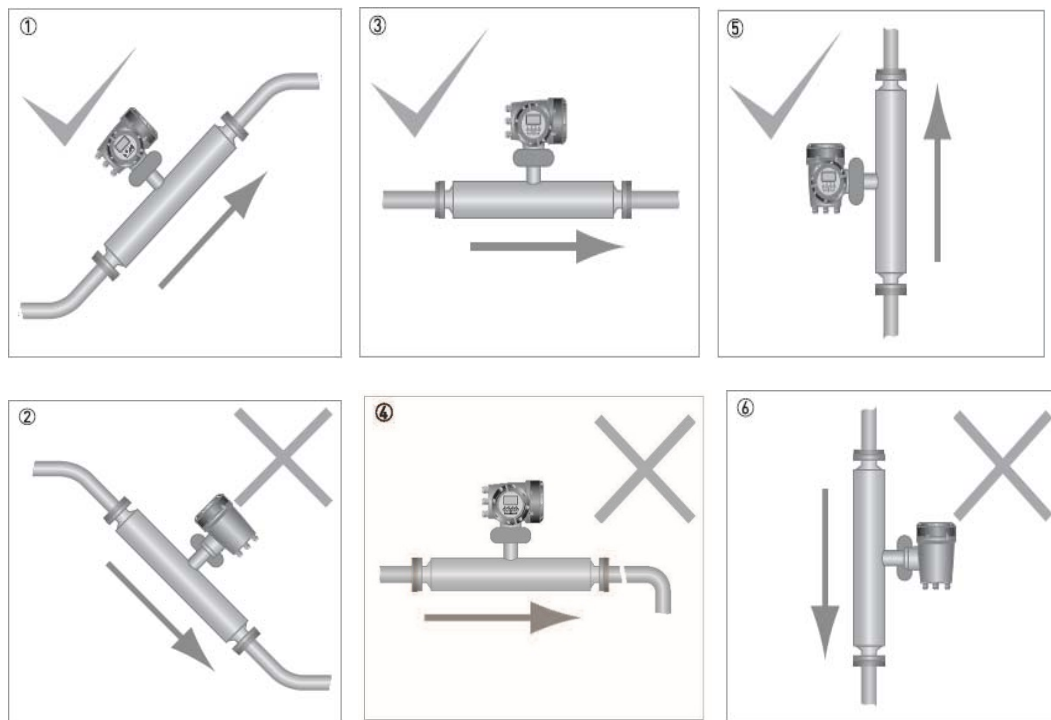
Figure 3 Installation of Flowmeters
