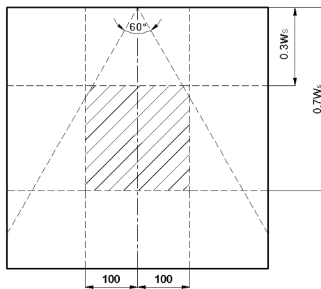
Figure B3 Effective Crack Arrest Zone
