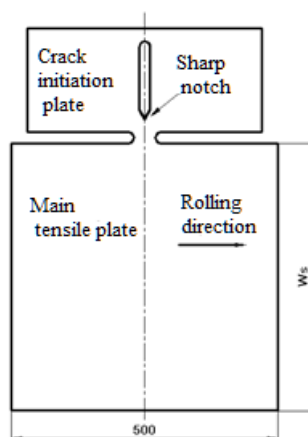
Figure B2 Shape and Size of Specimen
