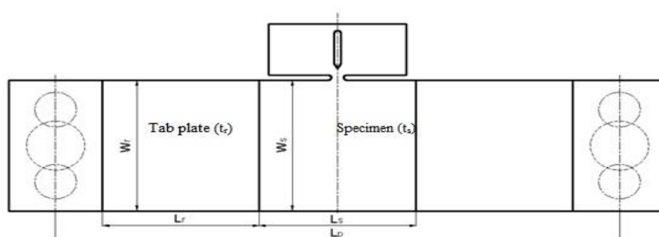
Figure B1 Specimen and Tab Plate
