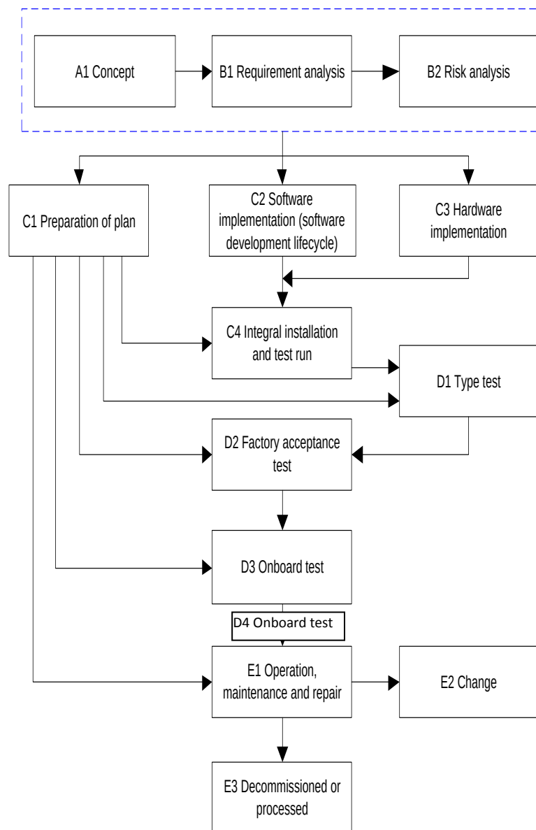
Fig. 6.1.1 System Lifecycle
