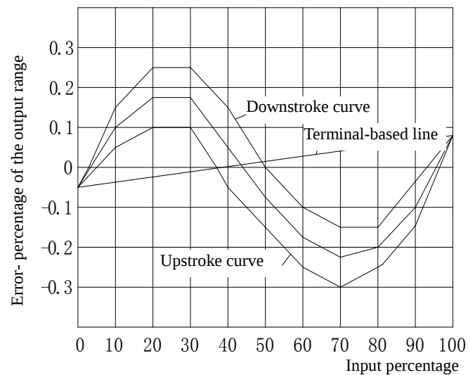
Fig. B1 Deviation curve
