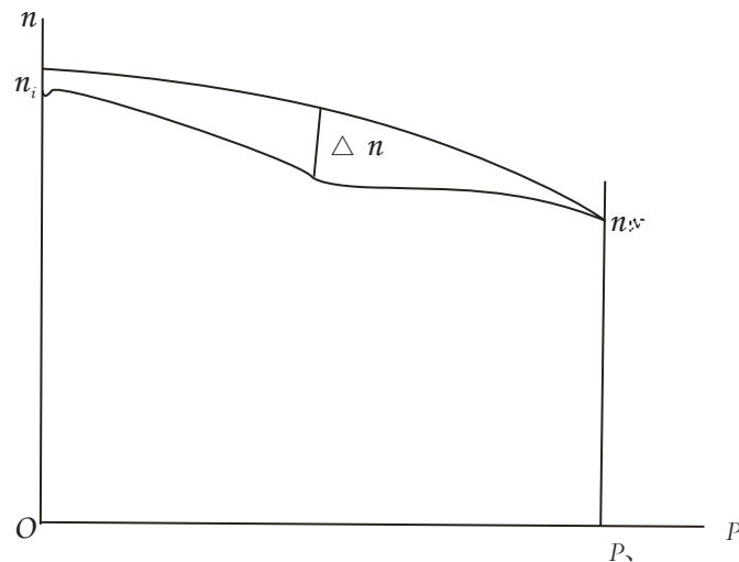
Figure 1.3.9 Insensitivity of Governing System
