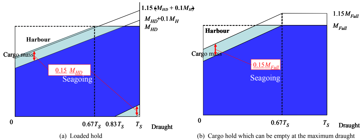
Figure 1: Example of mass curve for BC-A ships not having {No MP} assigned
