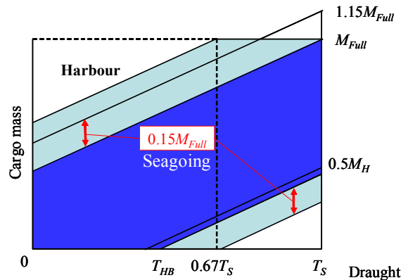
Figure 2.4: Example of mass curve for BC-B or BC-C ships Example of mass curve for BC-B and BC-C ships with having {No MP} assigned
