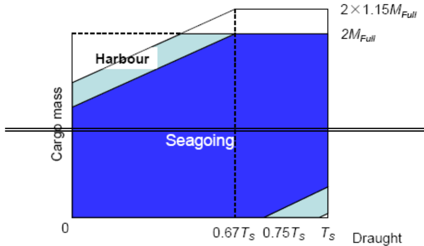
Figure 3: Example of mass curve for BC-B or BC-C ships
