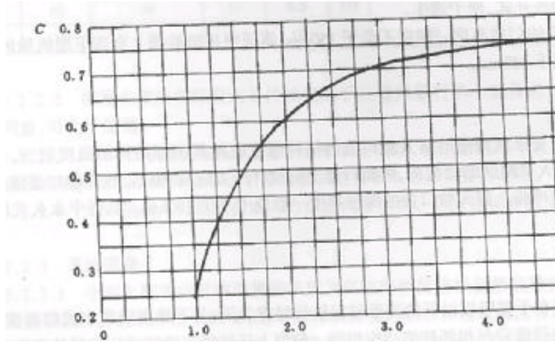
Fig. 2.4.2.1 Window aspect ratio = Long side length/ Short side length
