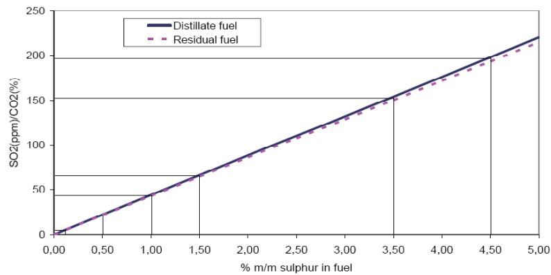
Figure 1 SO 2 /CO 2 ratio vs % sulphur in fuel
