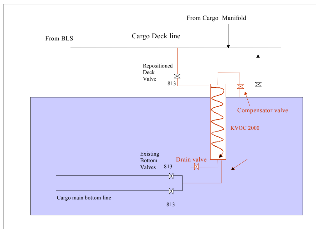
Pipeline Flow Plan for KVOG
